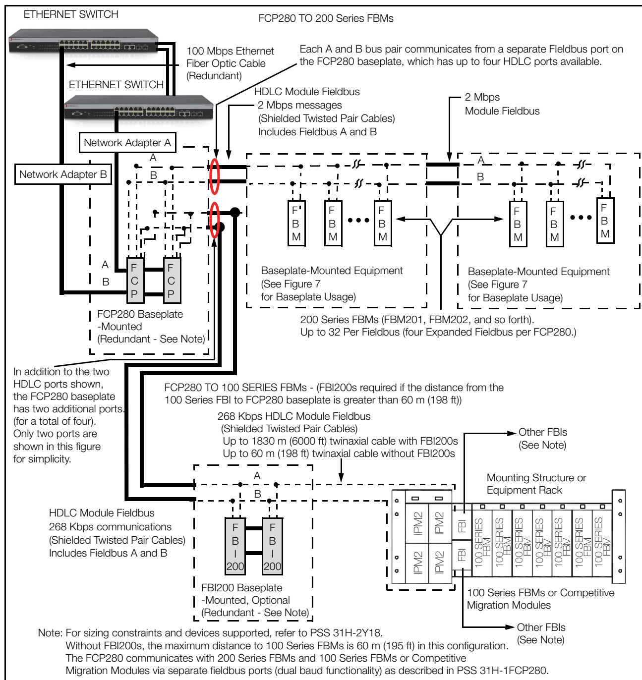
Figure 3. Standard 200 Series Subsystem, Typical FCP280 Configuration (Conceptual)
