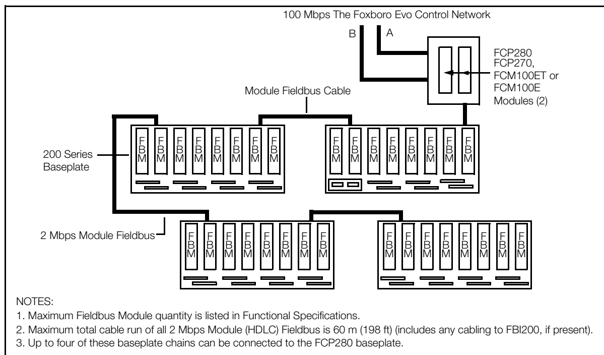
Figure 7. 200 Series Baseplate Implementation Example
