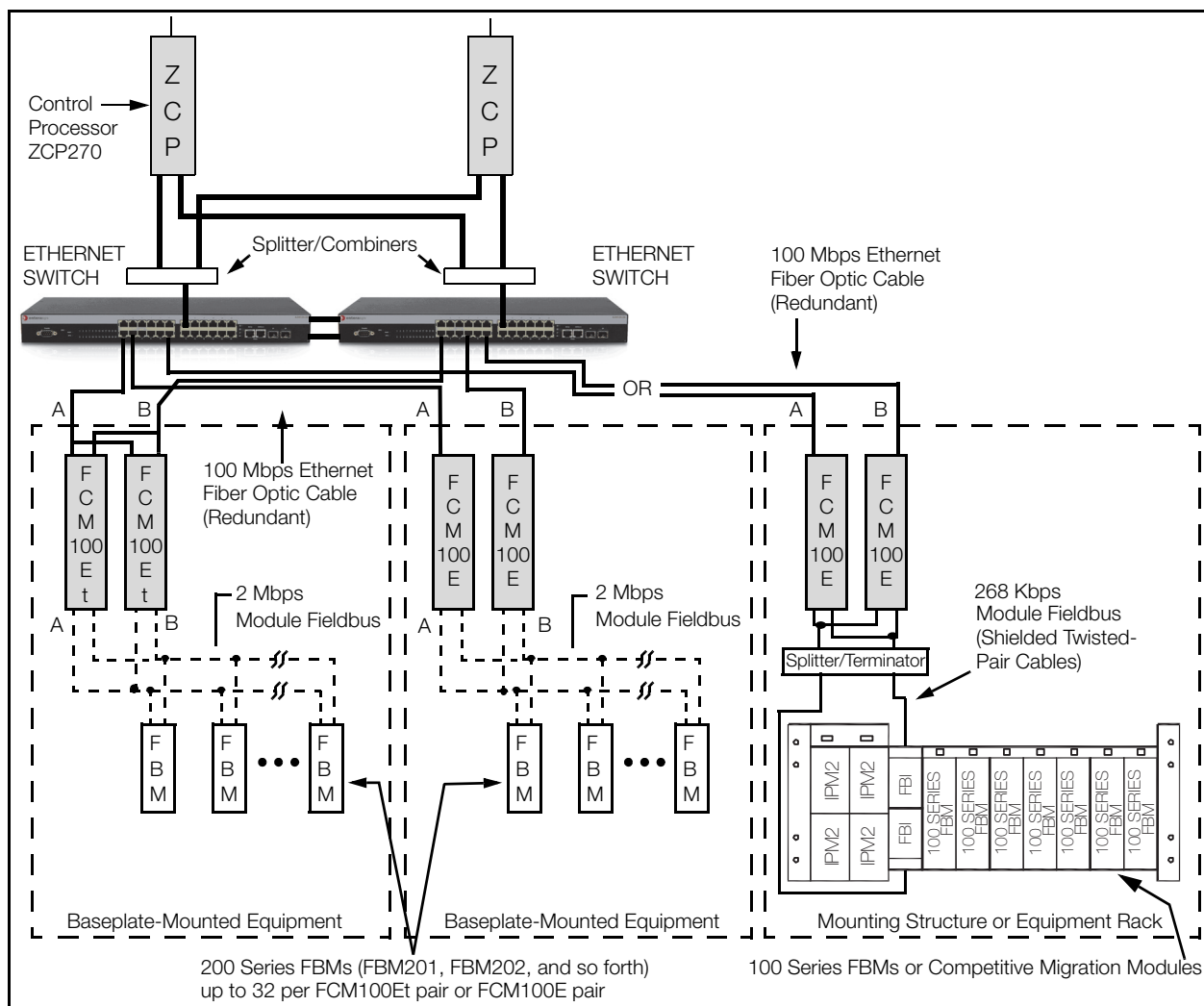
Figure 5. Standard 200 Series Subsystem, Typical FCM Configuration
