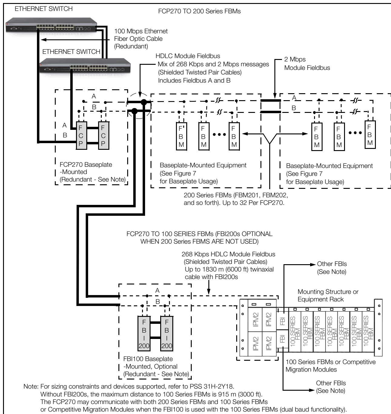
Figure 4. Standard 200 Series Subsystem, Typical FCP270 Configuration (Conceptual)
