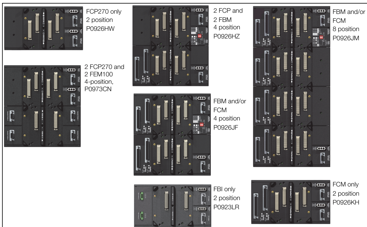
Figure 1. Vertically Mounted Standard 200 Series Baseplates (Selected Models)
