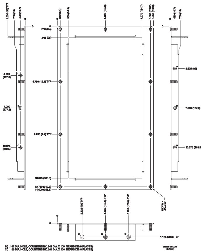
Figure 4 - Front Panel Mounting Bracket, P/N 9360107100
