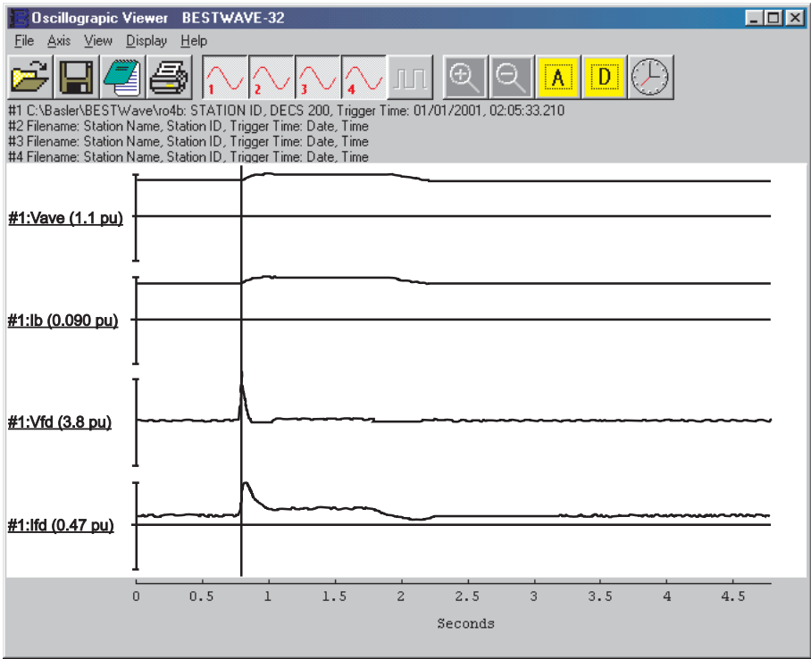
Figure 6 - BESTwave Oscillography
