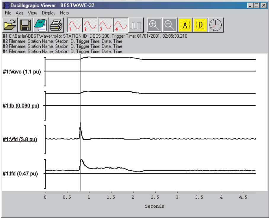
Figure 6 - BESTwave Oscillography
