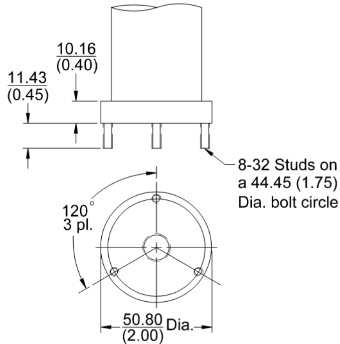
Figure 11: 9200 (C) and 74712 (B) Mounting Base
