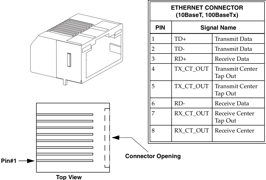
Figure A-4 Ethernet Connector and Pinout
