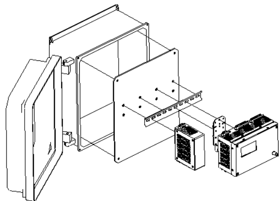
Figure 4: 1900/55 Replacement Kit
