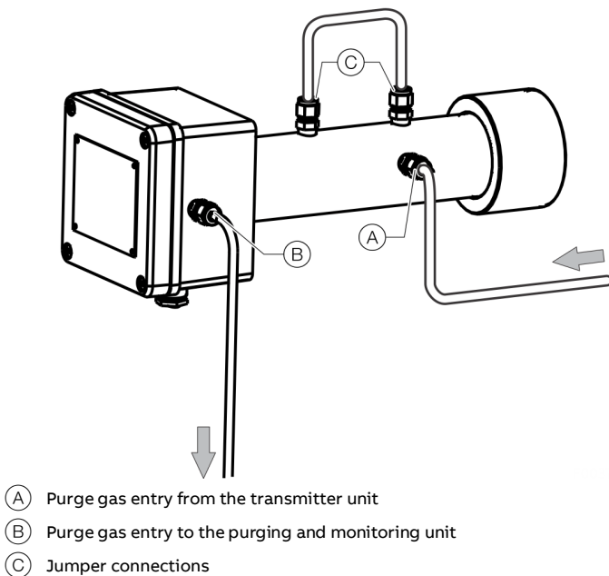
Figure 3: Purge gas connection to the receiver unit (N 2 as purge gas)
