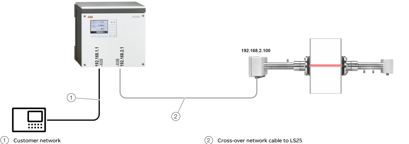
Figure 29: Ethernet connection – AO2000 with one laser analyzer
