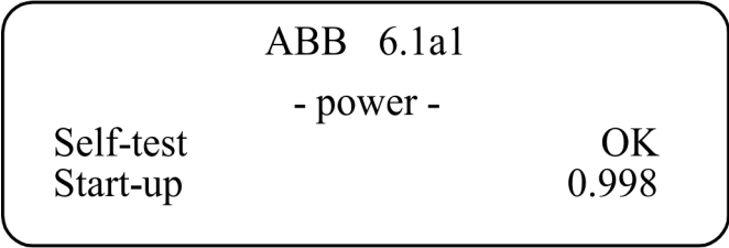
Figure 37: Start-up sequence
