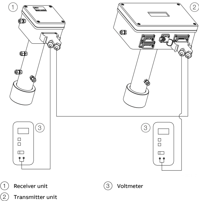
Figure 39: Measurement of adjustment voltage
