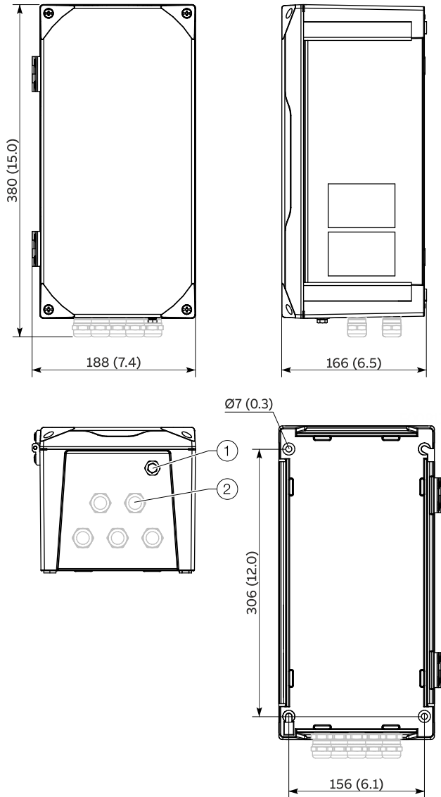
Figure 14: Dimensions in mm (in)
