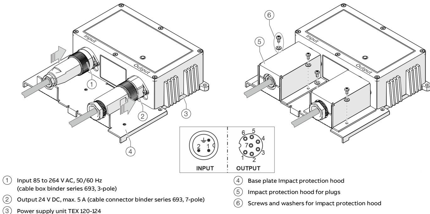
Figure 31: Power supply unit TEX 120-124
