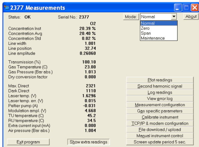
Figure 42: Menu “Measurements” (example)
