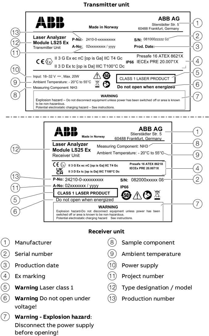
Figure 17: Name plate AO2000-LS25 (example, ATEX / IECEx version, Zone 2)
