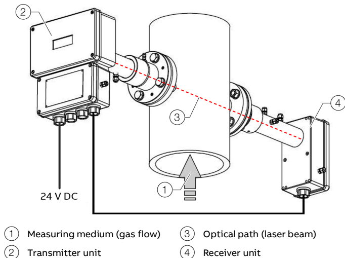
Figure 10: Measuring arrangement
