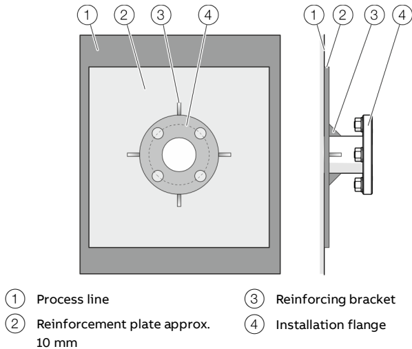
Figure 23: Reinforcement of the installation flanges
