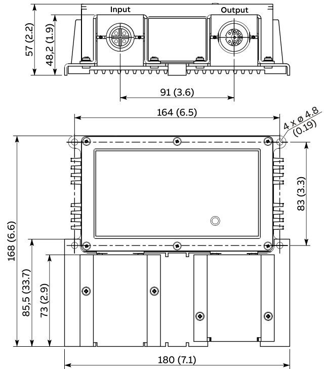
Figure 14: Dimensions in mm (in)
