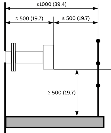
Figure 19: Transmitter and receiver installation tolerances
