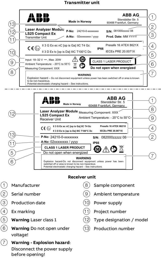
Figure 18: Name plate AO2000-LS25 Compact (example, ATEX / IECEx version, Zone 2)
