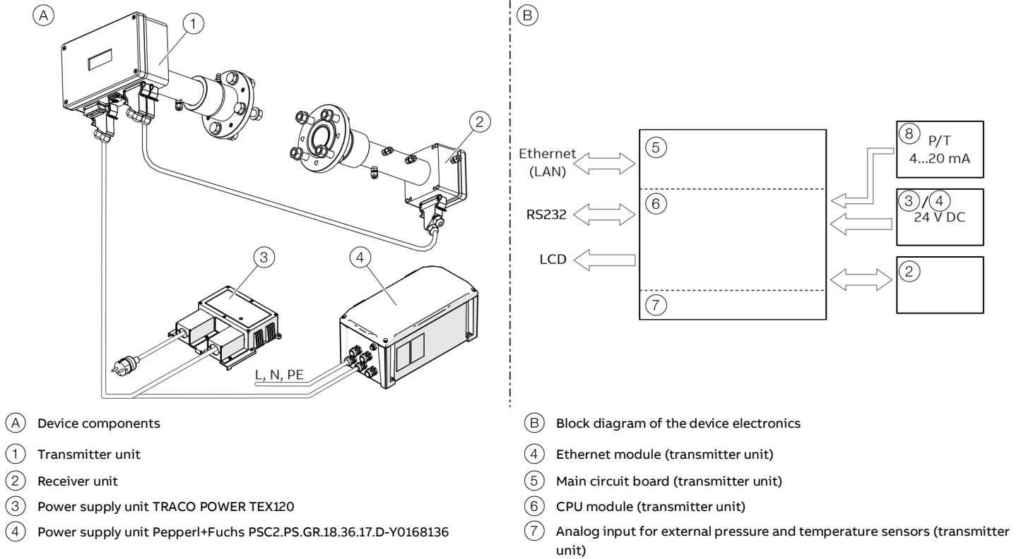
Figure 9: Overview AO2000-LS25
