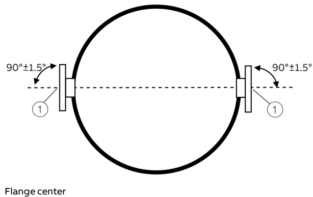
Figure 21: Alignment tolerances of the flange angle
